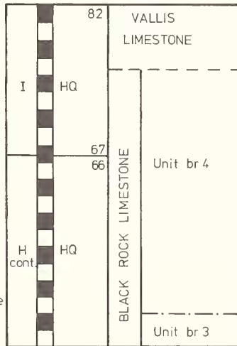
TEXT-FIG. 8. Location of sampled sections in Halecombe Quarry (ST 702 475) and notes on lithologies.
